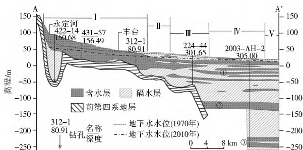
图 2 永定河冲洪积扇水文地质剖面 Fig. 2 Hydrogeological profile of the alluvial fan in the Yongding River
